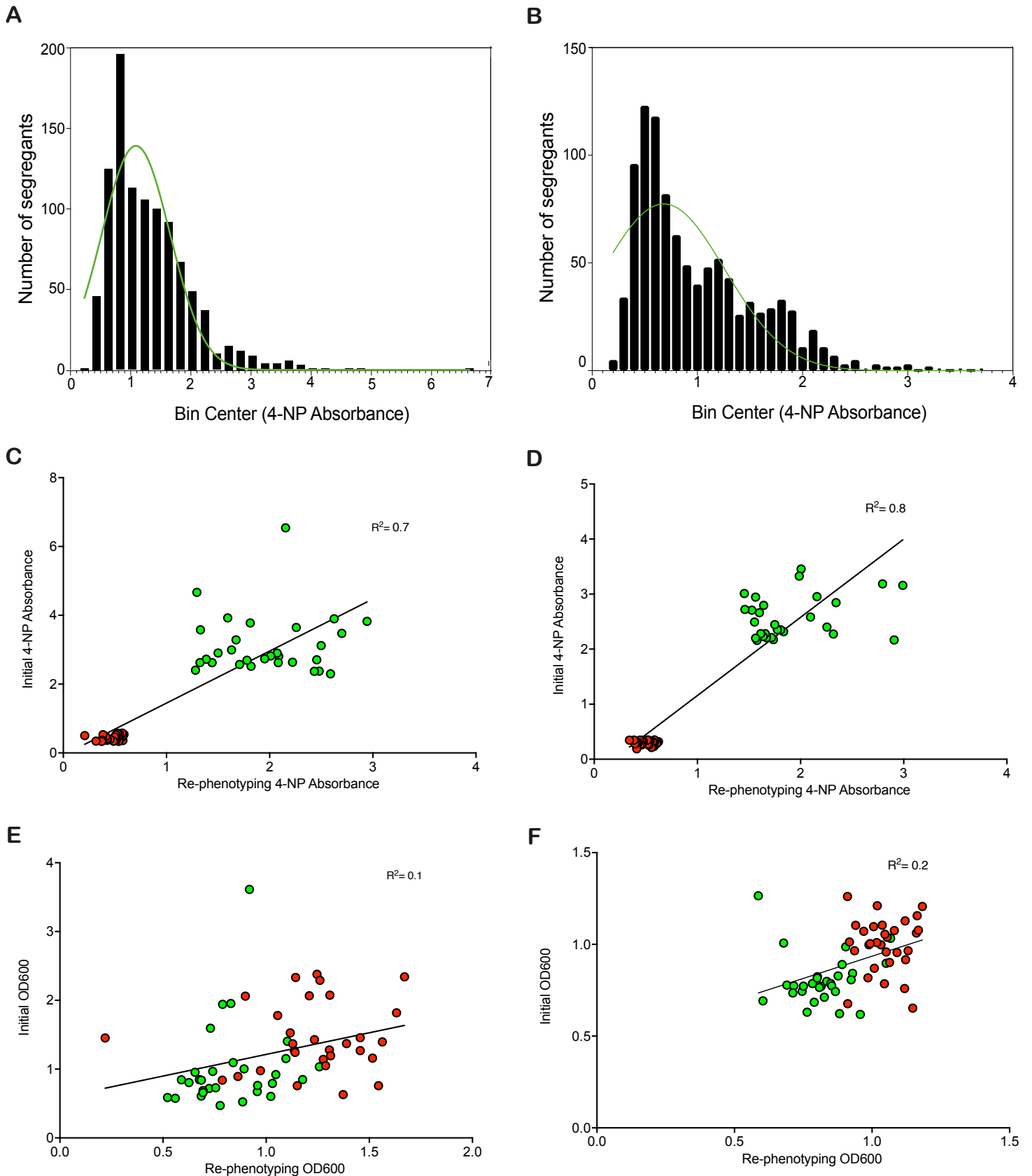
S3 Fig. Phenotypes of segregants.
